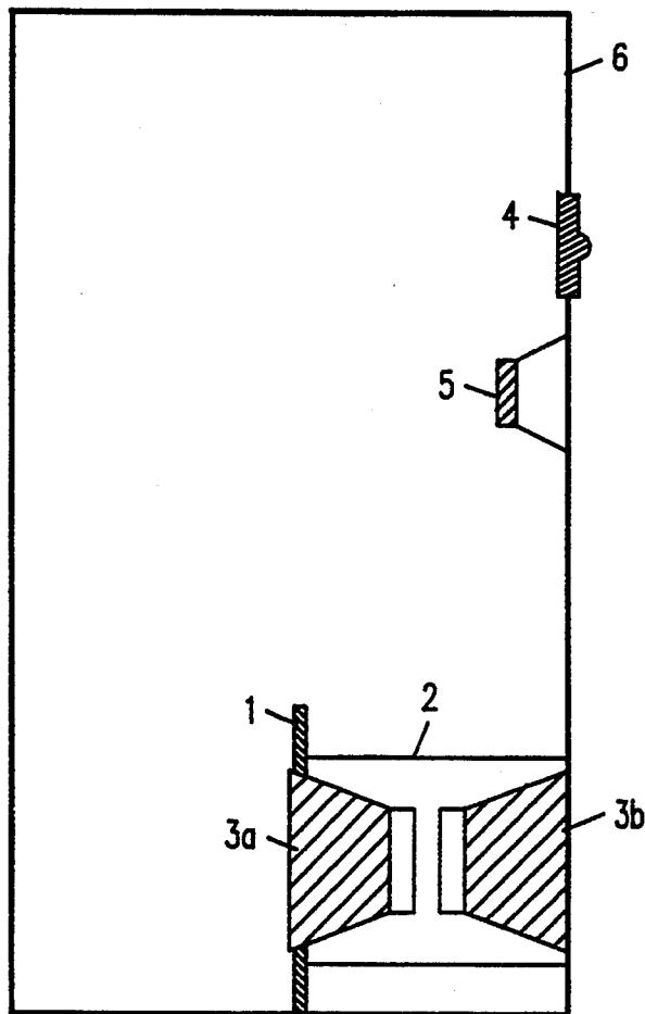
PRIOR ART FIG. 2
